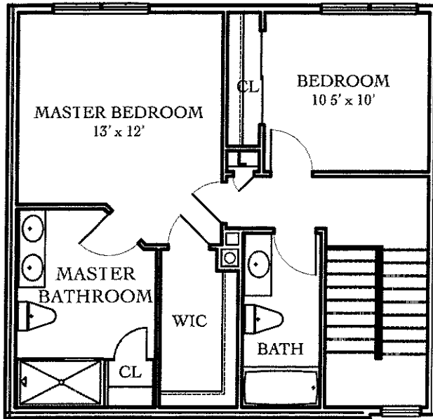
LEVEL THREE
